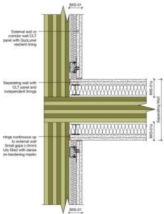
Typical junction (Plan) Separating Wall - External wall
